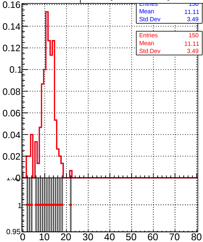
Legend: DQM_TT_mkFit-DQM_original (grey shaded area), DQM_TT_mkFit-DQM_modified2 (red line with markers)
