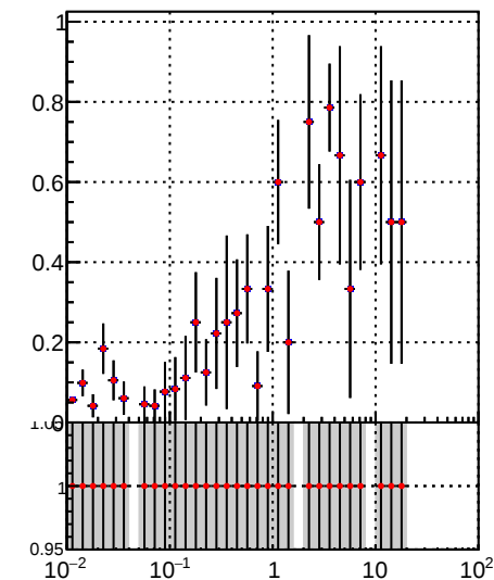
—•— DQM_TT_mkFit-DQM_original —•— DQM_TT_mkFit-DQM_modified2
