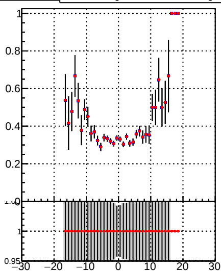
—•— DQM_TT_mkFit-DQM_original —•— DQM_TT_mkFit-DQM_modified2
