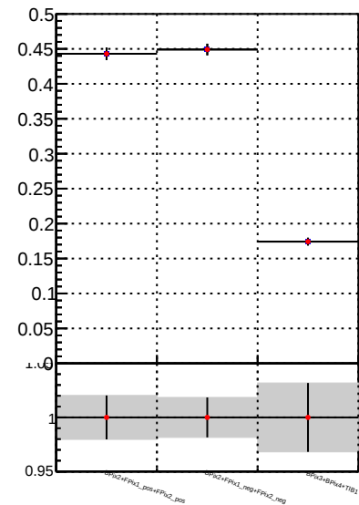
Fake rate vs. —•— DQM_TT_mkFit-DQM_original —•— DQM_TT_mkFit-DQM_modified2
