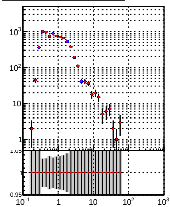
—●— DQM_TT_mkFit-DQM_original —●— DQM_TT_mkFit-DQM_modified2
