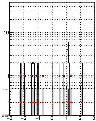
N of reco track vs \eta DQM TT mkFit-DQM original N of reco track vs \eta DQM TT mkFit-DQM modified2
