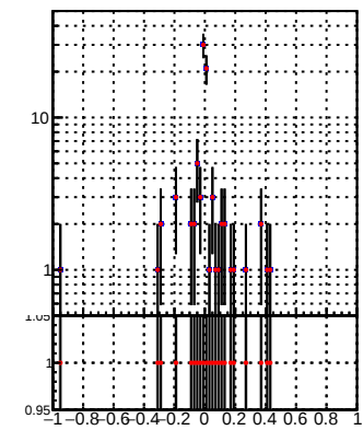
Legend: DQM_TT_mkFit-DQM_original (grey shaded area) DQM_TT_mkFit-DQM_modified2 (red line)
