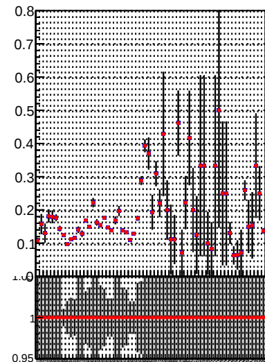
Fake rate vs. —●— DQM_TT_mkFit-DQM_original —●— DQM_TT_mkFit-DQM_modified2
