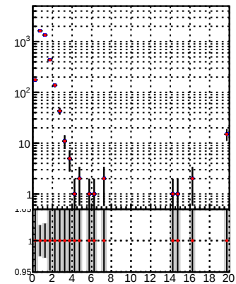
N of reco track vs. \chi^2 — mkFit-DQM_original — mkFit-DQM_modified2
