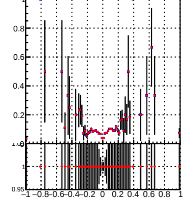
fake+duplicates vs dxy(PV)
