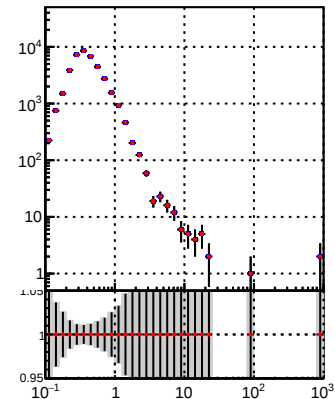
—•— DQM_TT_mkFit-DQM_original —•— DQM_TT_mkFit-DQM_modified2
