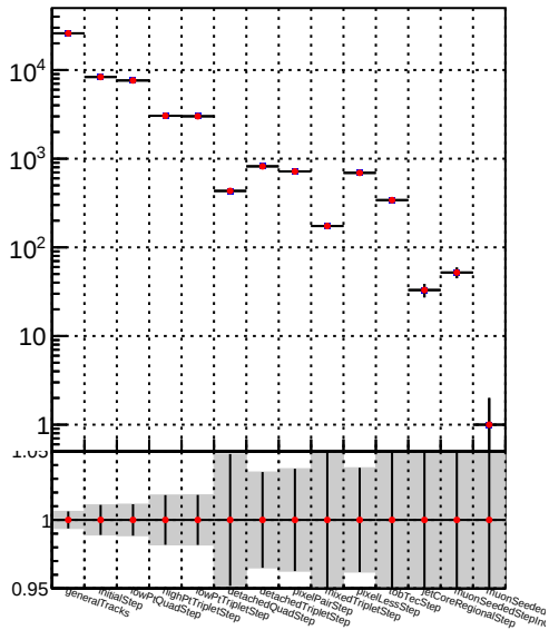
Number —●— DQM_TT__mkFit-DQM_modified2
