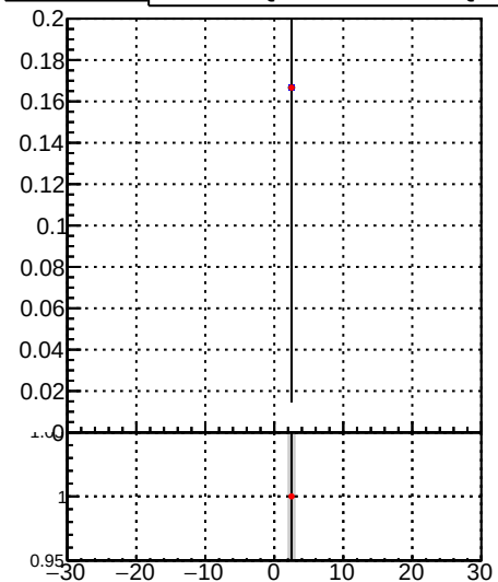
Fake rate vs v Legend: DQM_TT_mkFit-DQM_original (grey line with blue dots) DQM_TT_mkFit-DQM_modified2 (red line with red dots)
