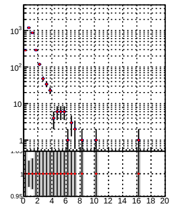
N of reco track vs. \chi^2 for DQM TT mkFit-DQM_original and DQM TT mkFit-DQM_modified2
