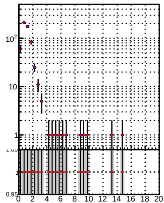
N of reco track vs. \chi^2 for different track types
