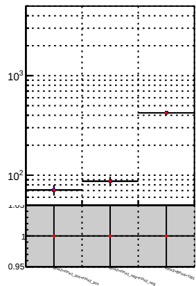
N of reco track vs. \chi^2 for different track types
