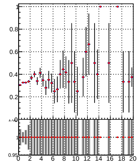
Fake rate vs. — \bullet DQM_TT_mkFit-DQM_original — \bullet DQM_TT_mkFit-DQM_modified2
