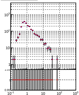
—●— DQM_TT_mkFit-DQM_original —●— DQM_TT_mkFit-DQM_modified2
