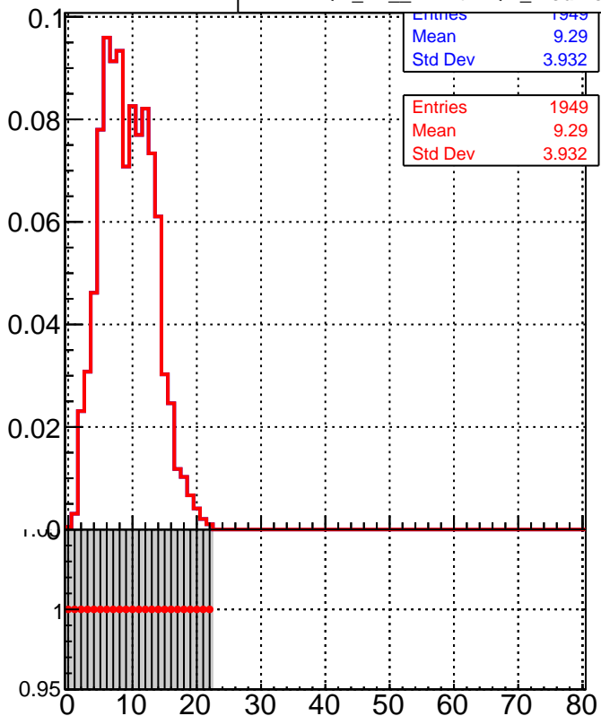
█ DQM_TT_mkFit-DQM_original █ DQM_TT_mkFit-DQM_modified2
