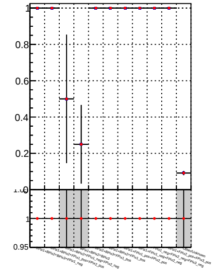
Fake rate vs. DQM_TT_mkFit-DQM_original DQM_TT_mkFit-DQM_modified2
