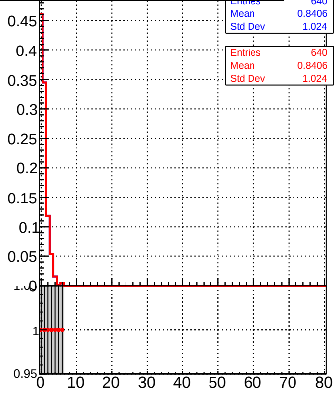
Legend for bottom row plots: DQM_TT_mkFit-DQM_original (Blue line with squares) DQM_TT_mkFit-DQM_modified2 (Red line with circles)
