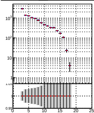
DQM_TT_mkFit-DQM_original DQM_TT_mkFit-DQM_modified2
