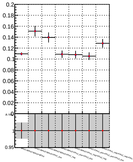
Fake rate vs. \bullet DQM_TT_mkFit-DQM_original \bullet DQM_TT_mkFit-DQM_modified2
