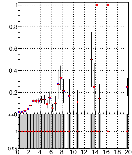
Fake rate vs. —•— DQM_TT mkFit-DQM_original —•— DQM_TT mkFit-DQM_modified2
