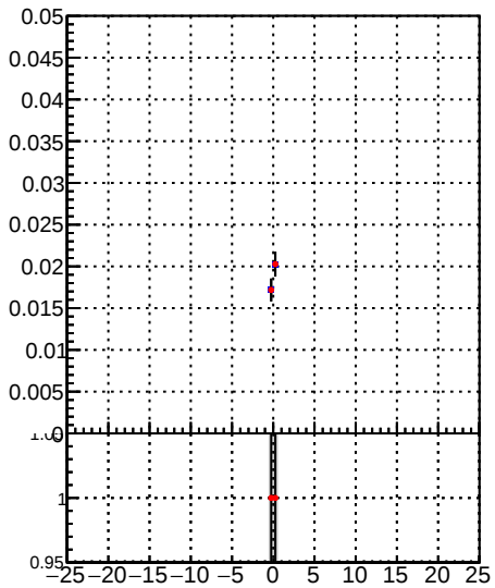
Fake rate vs d —•— DQM_TT_mkFit-DQM_original —•— DQM_TT_mkFit-DQM_modified2
