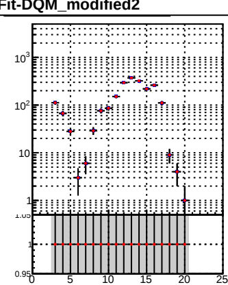
■ DQM_TT_mkFit-DQM_original ● DQM_TT_mkFit-DQM_modified2
