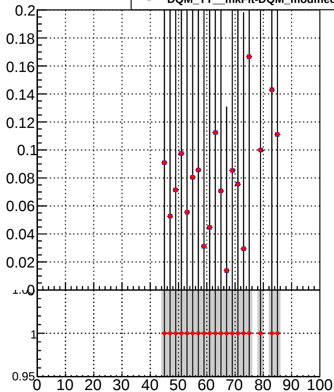
—●— DQM_TT_mkFit-DQM_original —●— DQM_TT_mkFit-DQM_modified2
