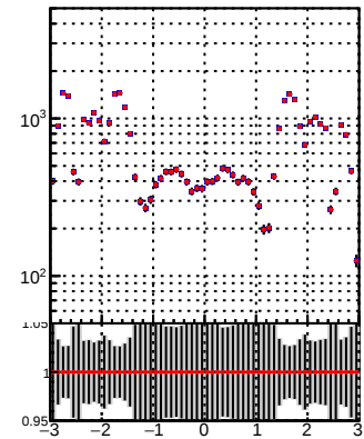
DQM_TT mkFit-DQM_original DQM_TT mkFit-DQM_modified2
