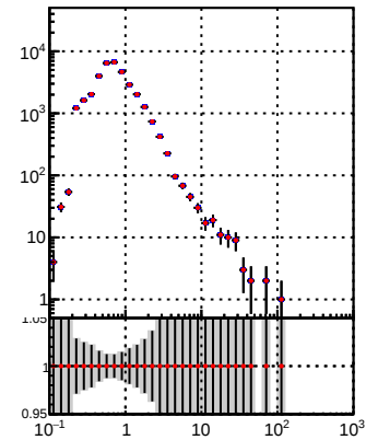
DQM_TT mkFit-DQM_original DQM_TT mkFit-DQM_modified2
