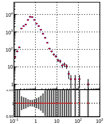
DQM_TT mkFit-DQM_original DQM_TT mkFit-DQM_modified2
