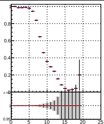
Legend: DQM_TT_mkFit-DQM_original (grey histogram), DQM_TT_mkFit-DQM_modified2 (red line with dots)
