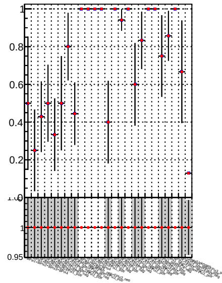
Fake rate vs. — DQM TT mkFit-DQM_original — DQM TT mkFit-DQM_modified2
