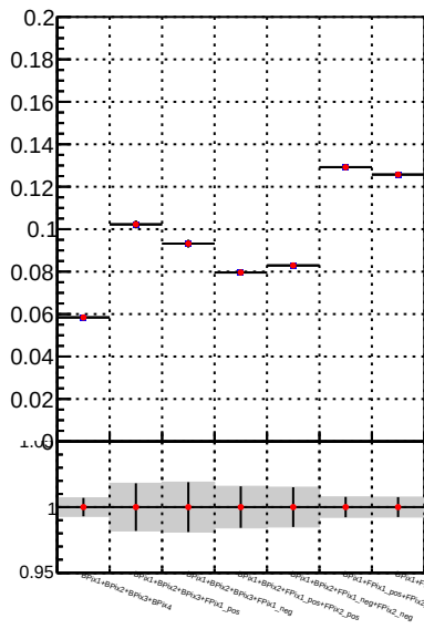
Fake rate vs. —•— DQM TT mkFit-DQM_original —•— DQM TT mkFit-DQM_modified2
