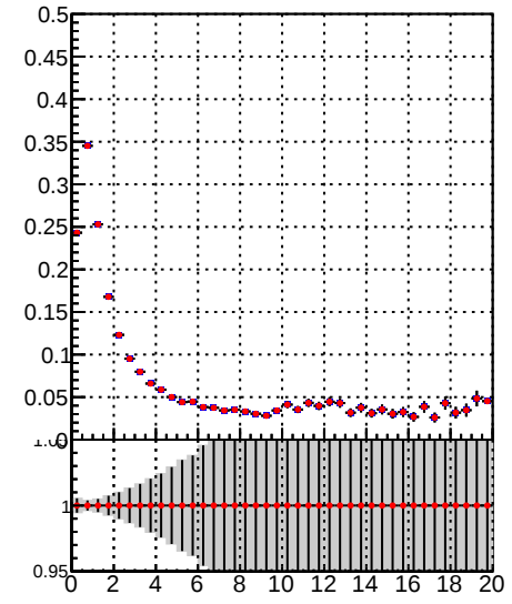
Fake rate vs. —●— DQM_TT_mkFit-DQM_original —●— DQM_TT_mkFit-DQM_modified2
