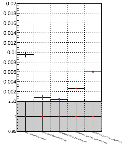
DQM_TT_mkFit-DQM_original DQM_TT_mkFit-DQM_modified2
