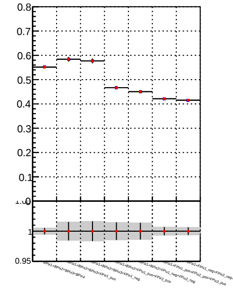
DQM_TT_mkFit-DQM_original DQM_TT_mkFit-DQM_modified2
