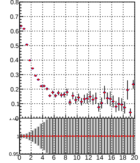
DQM_TT_mkFit-DQM_original DQM_TT_mkFit-DQM_modified2
