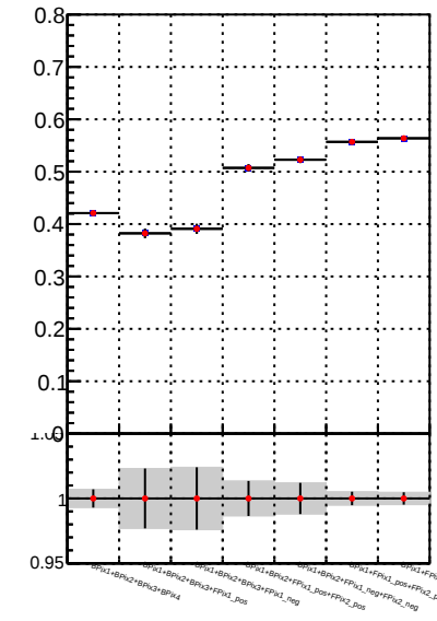
DQM_TT_mkFit-DQM_original DQM_TT_mkFit-DQM_modified2
