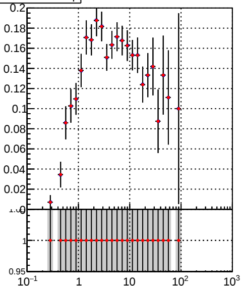
— DQM_TT_mkFit-DQM_original — DQM_TT_mkFit-DQM_modified2
