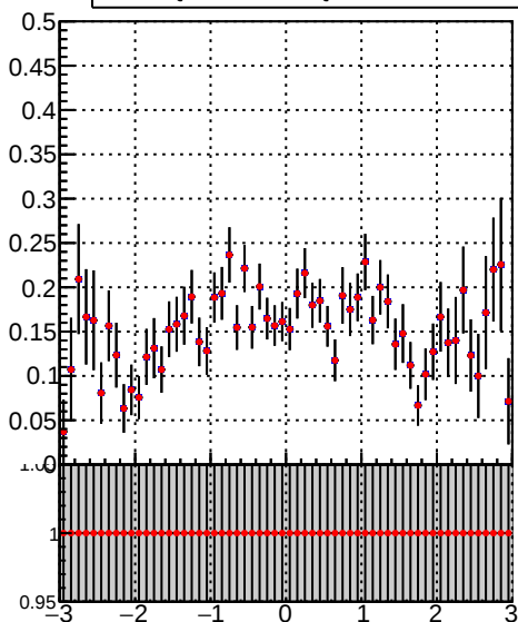
— DQM_TT_mkFit-DQM_original — DQM_TT_mkFit-DQM_modified2
