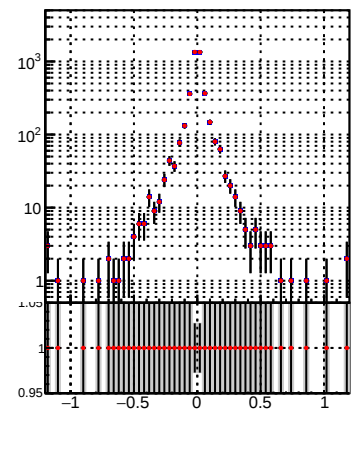
N of associated tracks (simToReco) vs dz(PV) zoomed
