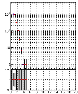
N of reco track vs. \chi^2 (mkFit-DQM_original vs mkFit-DQM_modified2)
