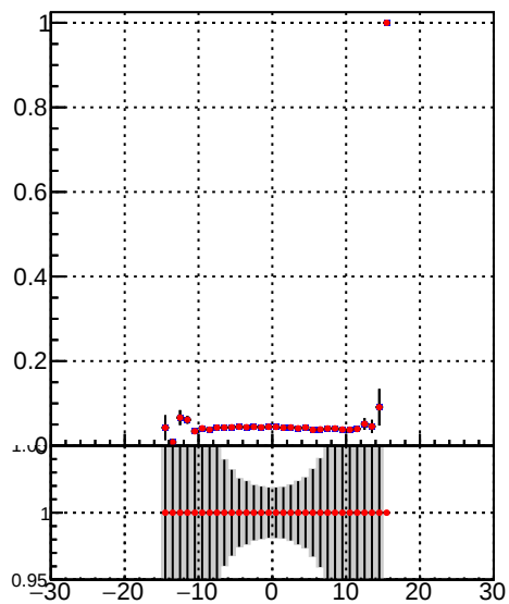
Efficiency vs. sim PV z Legend: — DQM_TT_mkFit-DQM_original — DQM_TT_mkFit-DQM_modified2
