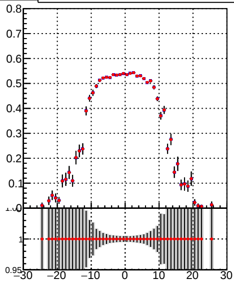
Efficiency vs. sim PV z Legend: — DQM_TT_mkFit-DQM_original — DQM_TT_mkFit-DQM_modified2
