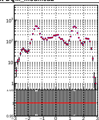
—●— DQM_TT_mkFit-DQM_original —●— DQM_TT_mkFit-DQM_modified2
