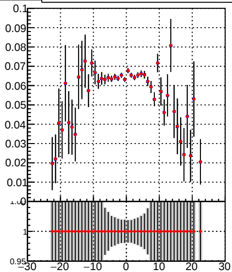
Efficiency vs. sim PV z — DQM_TT_mkFit-DQM_original — DQM_TT_mkFit-DQM_modified2
