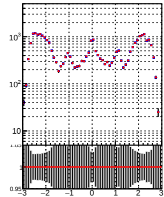
—●— DQM_TT_mkFit-DQM_original —●— DQM_TT_mkFit-DQM_modified2
