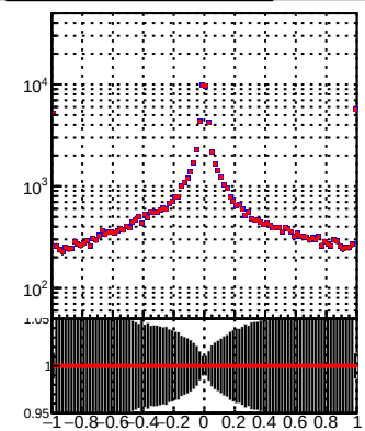
Legend: DQM_TT_mkFit-DQM_original (black histogram) DQM_TT_mkFit-DQM_modified2 (red dashed line)
