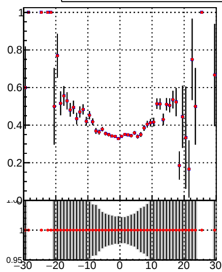
—•— DQM_TT_mkFit-DQM_original —•— DQM_TT_mkFit-DQM_modified2
