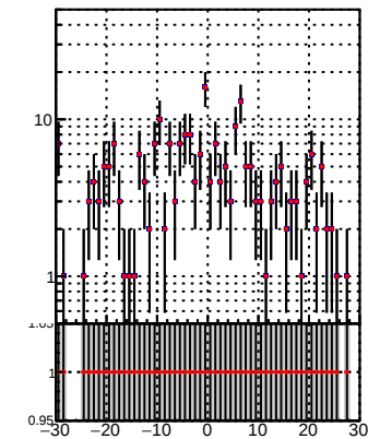
N of associated (recoToSim) loopier tracks vs dz
