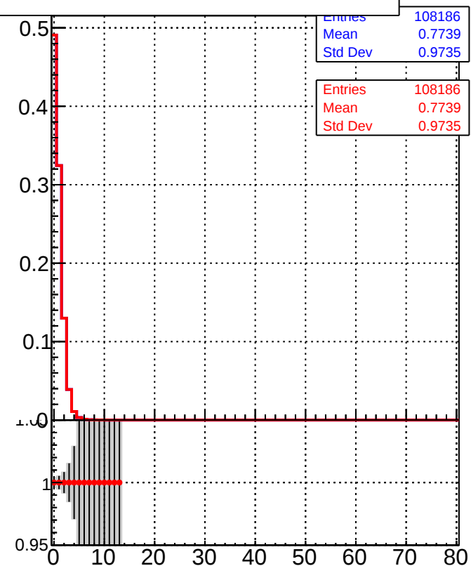
Legend: ■ DQM_TT_mkFit-DQM_original ● DQM_TT_mkFit-DQM_modified2
