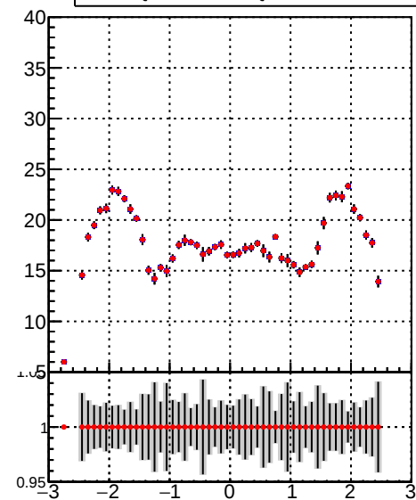
mean hit — DQM_TT_mkFit-DQM_original — DQM_TT_mkFit-DQM_modified2
