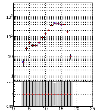
—•— DQM_TT_mkFit-DQM_original —•— DQM_TT_mkFit-DQM_modified2
