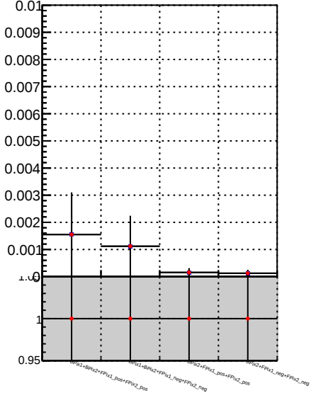
Fake rate vs. \text{DQM\_TT\_mkFit-DQM\_original} \text{DQM\_TT\_mkFit-DQM\_modified2}
