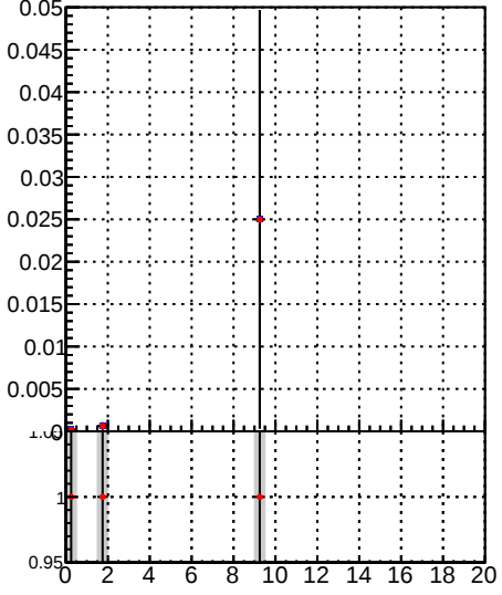
Fake rate vs. \text{DQM\_TT\_mkFit-DQM\_original} \text{DQM\_TT\_mkFit-DQM\_modified2}
