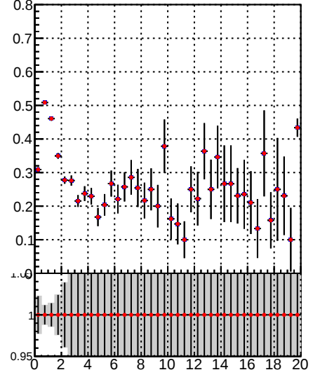
Fake rate vs. \text{DQM\_TT\_mkFit-DQM\_original} \text{DQM\_TT\_mkFit-DQM\_modified2}
