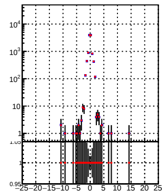
DQM_TT_mkFit-DQM_original DQM_TT_mkFit-DQM_modified2
