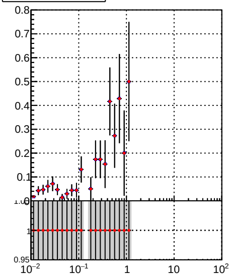
Fake rate vs v DQM_TT_mkFit-DQM_original DQM_TT_mkFit-DQM_modified2
