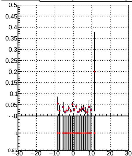
Fake rate vs v DQM_TT_mkFit-DQM_original DQM_TT_mkFit-DQM_modified2
