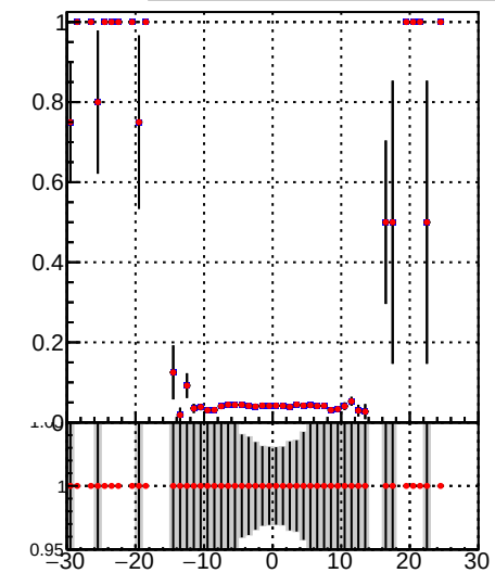
—•— DQM_TT_mkFit-DQM_original —•— DQM_TT_mkFit-DQM_modified2
