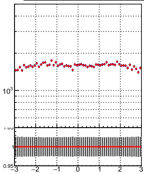
■ DQM_TT_mkFit-DQM_original ● DQM_TT_mkFit-DQM_modified
