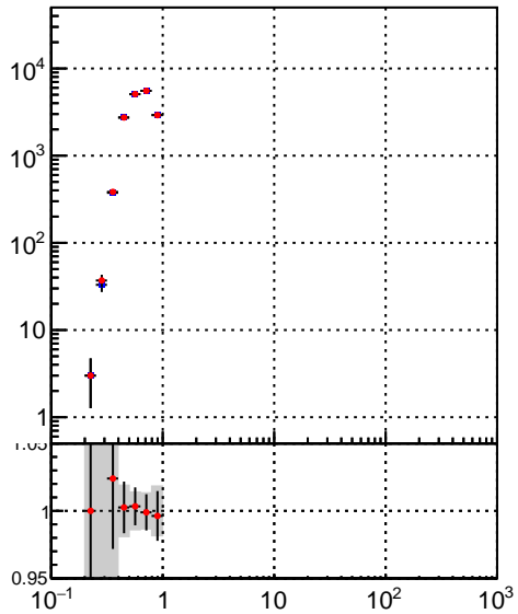
■ DQM_TT_mkFit-DQM_original ● DQM_TT_mkFit-DQM_modified
